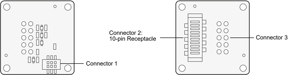
Fig. 1: dart I/O Board 2 Top and Bottom
