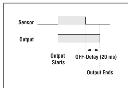
Figure 4. Output OFF-delay: Output continues for 20 ms after sensing stops
