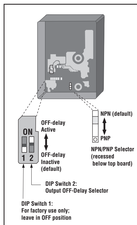
Figure 5. Selector switches: Output OFF-Delay and NPN/PNP output select
