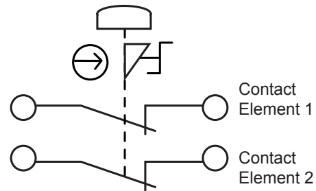
E-Stop wiring diagram
