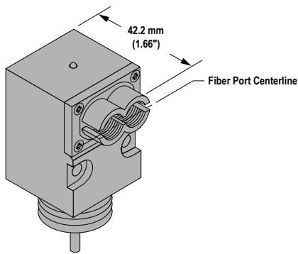
Figure 5. Glass Fiber Optic Models (model suffix F)
