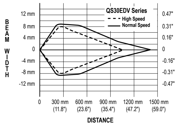
Figure 2. Beam Pattern
