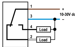
PNP
