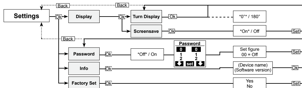
Figure 17. Settings Menu
