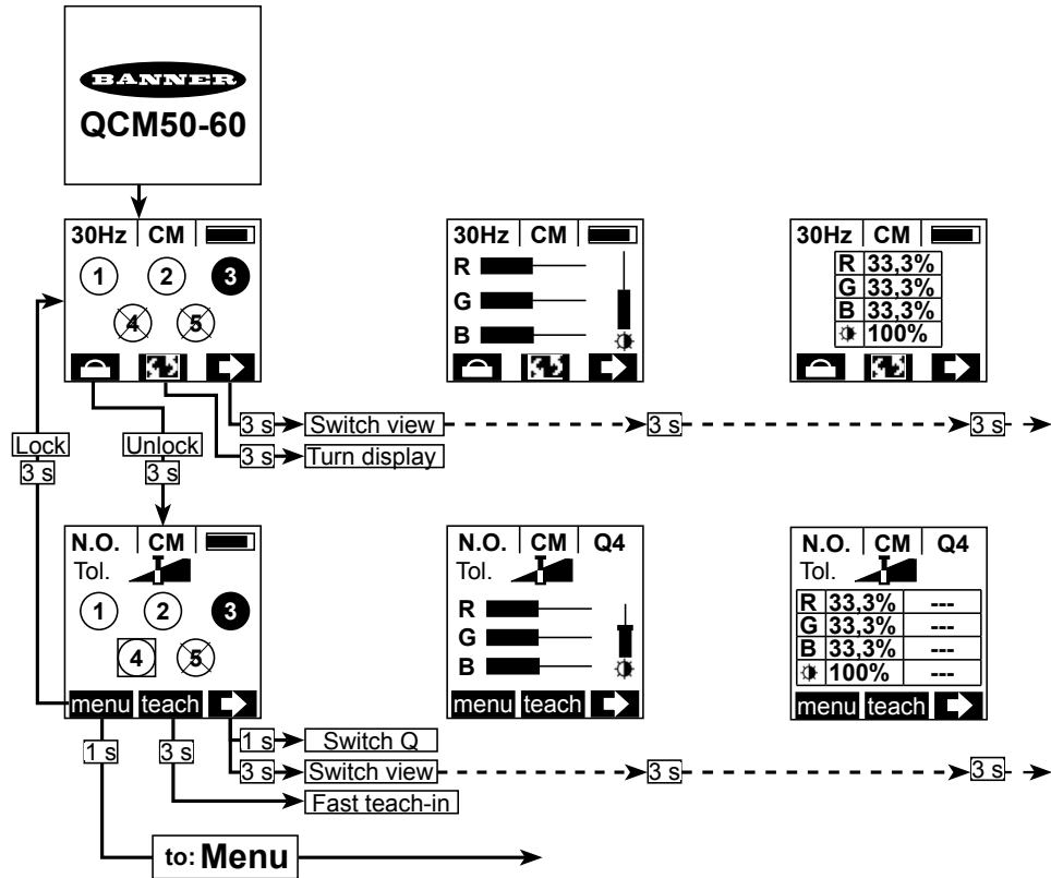
Figure 12. Top Level Menu
