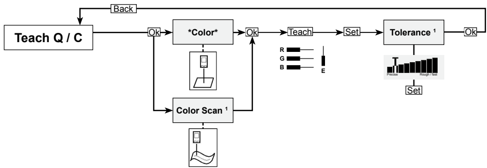
Figure 7. Teach Menu
