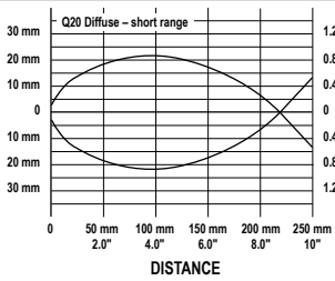
Beam Pattern
