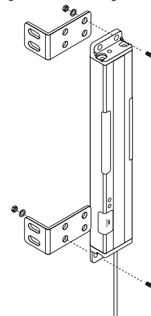
Figure 6. PVD Mounting Hardware
