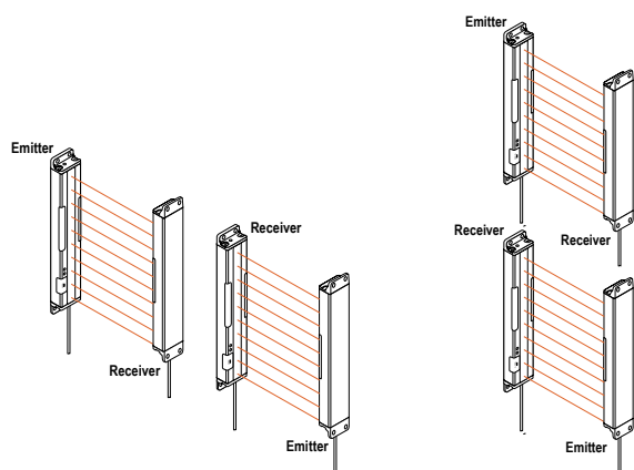
Figure 1. Example—Correct Positions
