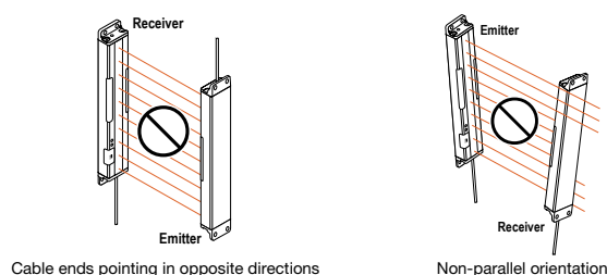
Figure 2. Example—Incorrect Positions
