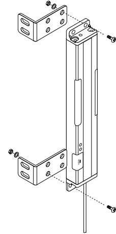
Figure 4. Mounting Hardware
