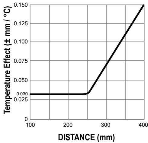
Figure 28. Temperature Effect
