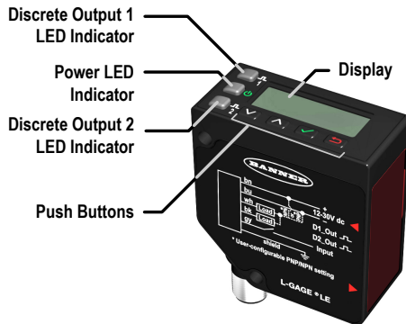
Figure 1. LE Dual Discrete Sensor Features
