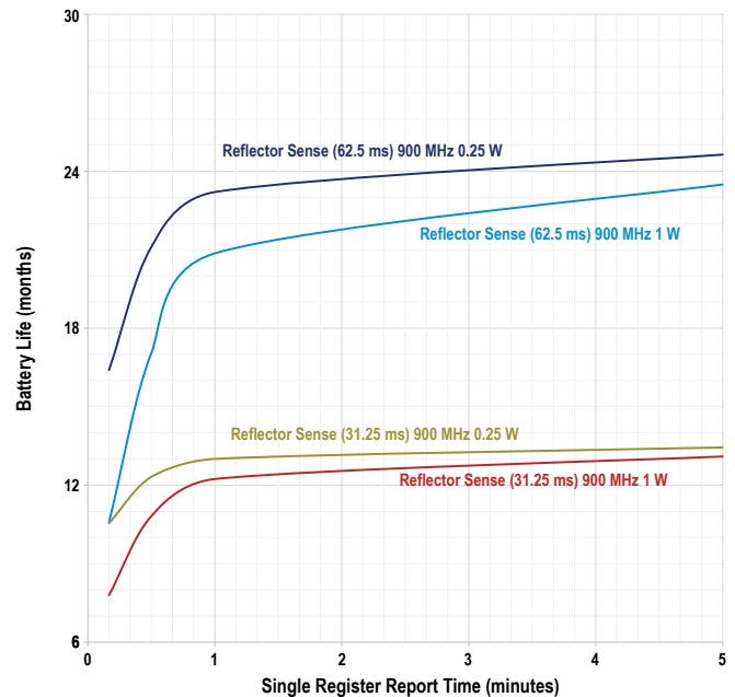
Figure 8. 900 MHz Radios
