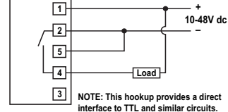
Alternative Low Saturation Sinking (NPN) Hookup
