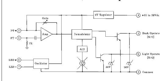
Functional Schematic, MA3 Amplifier
