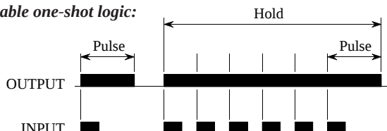
Retriggerable one-shot logic:
