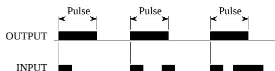
Non-retriggerable one-shot logic:
