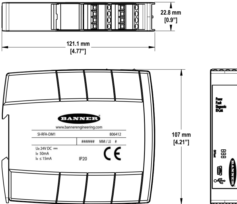
Figure 5. SI-RF-DM1 Module
