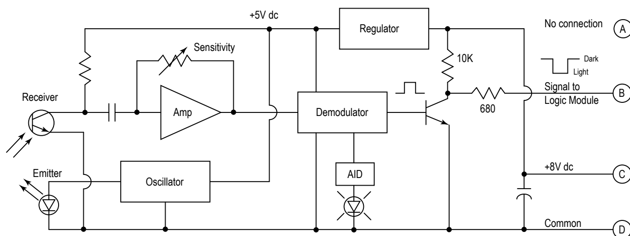
Figure 1. Functional Schematic
