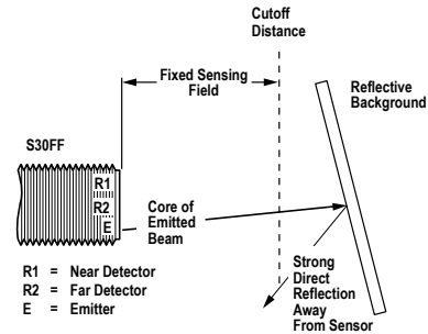
Figure 4. Reflective Background - Solution
