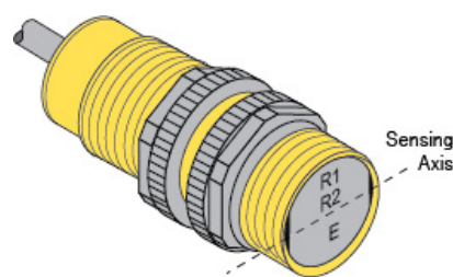
Figure 2. Fixed-Field Sensing Axis
