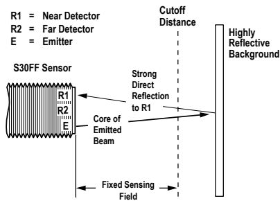
Figure 3. Reflective Background - Problem
