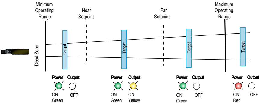
TEACH Interface
