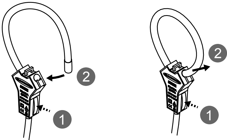
Installing the 50mm current transformer loop model
