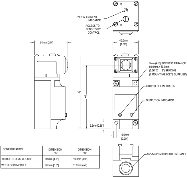
Figure 3. Dimensions for the FF models
