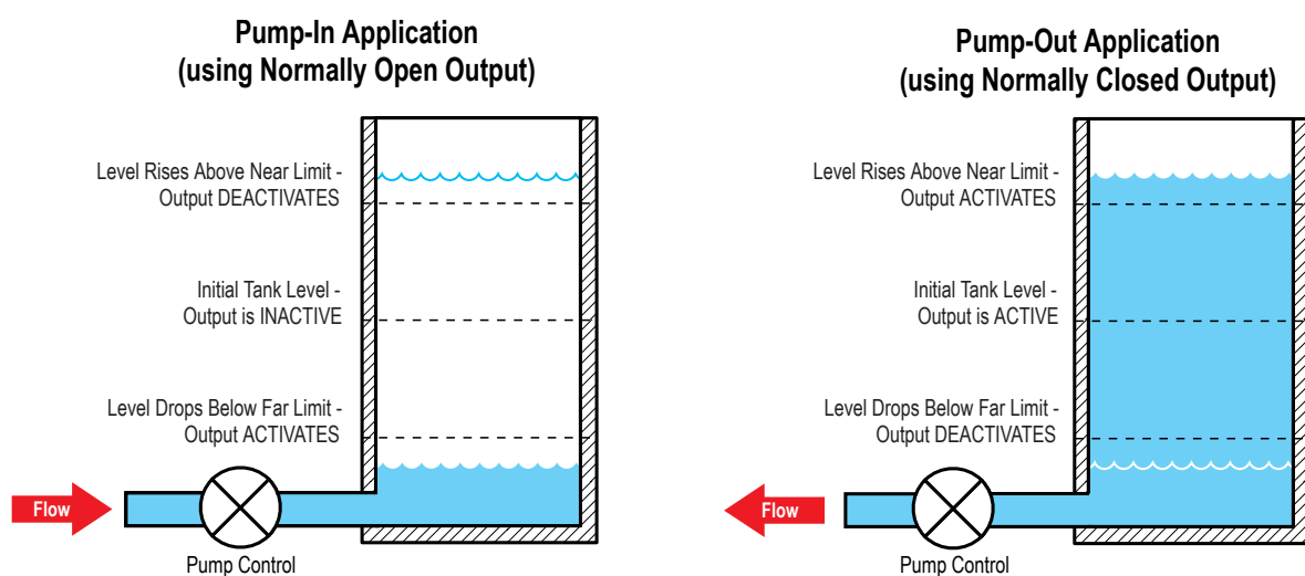
Figure 5. Fill-Level Control
