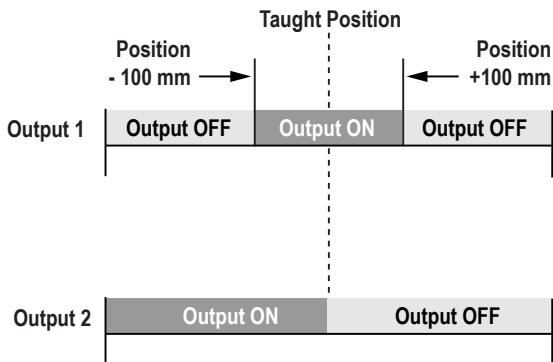
Figure 7. Using simultaneous auto-window/background suppression (normally open illustrated)
