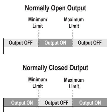
Figure 4. Teaching independent minimum and maximum limits
