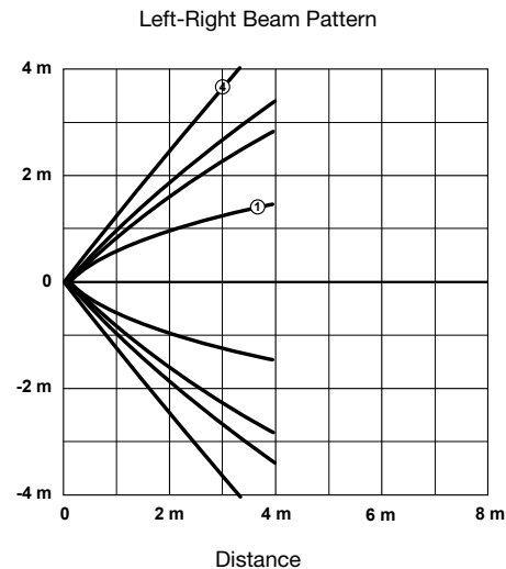
Typical Beam Pattern (with 4 different targets) at highest sensitivity level
