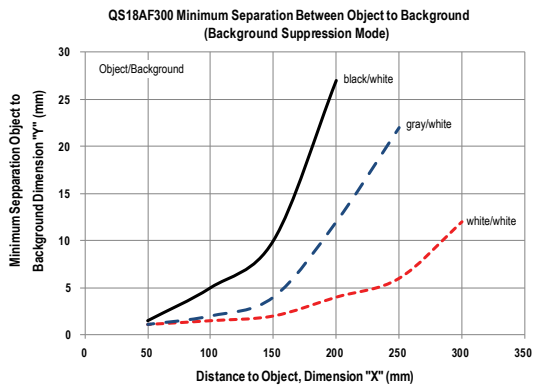
Figure 7. Minimum Separation Distance Between Object and Background: Background Suppression Mode
