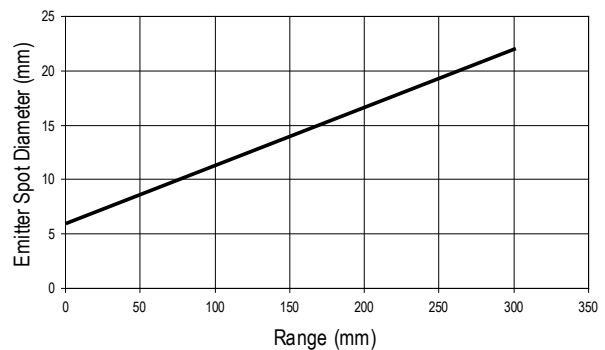
Figure 6. Typical Emitter Spot Diameter vs. Distance
