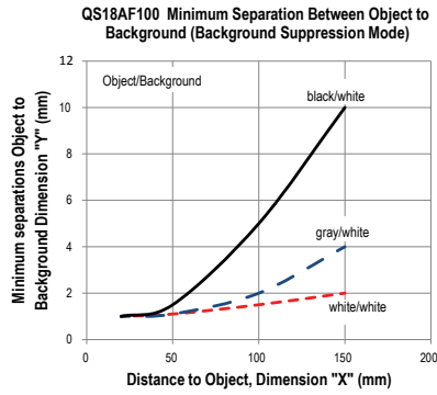
Figure 3. QS18AF100 minimum separation between object and background
