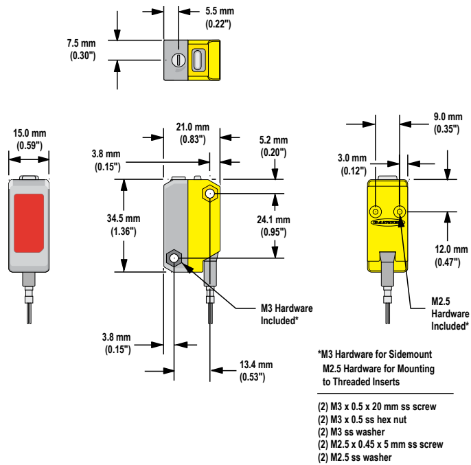
Figure 12. QS18AF Dimensions
