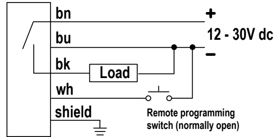
Figure 7. PNP (Sourcing) Output Models
