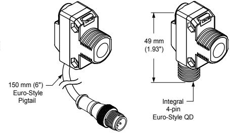
Figure 12. M12 QD models
