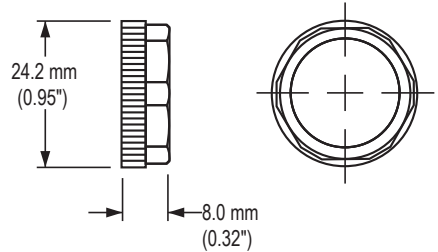
Figure 13. Locknut (included with all models)
