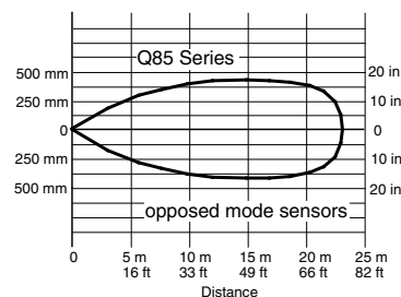
Beam Pattern
