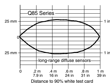
Beam Pattern
