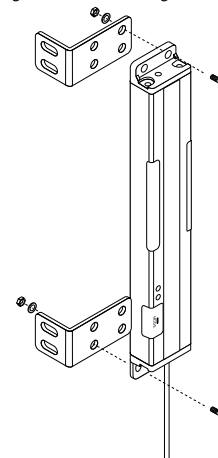
Figure 6. PVD Mounting Hardware
