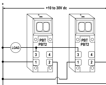
Figure 9. Parallel Wiring to a Common Load (requiring NPN current)
