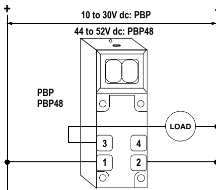
Figure 8. Wiring to DC Relay or Solenoid (using PNP output)
