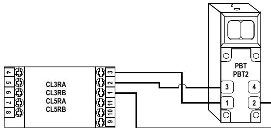
Figure 13. Wiring to MAXI-AMP Logic Module
