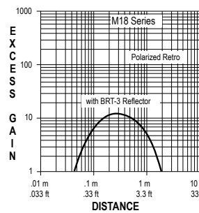
Excess Gain
