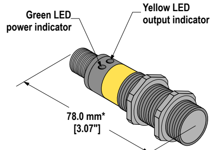
Figure 15. Models with 4-pin M12/Euro-style Quick Disconnect
