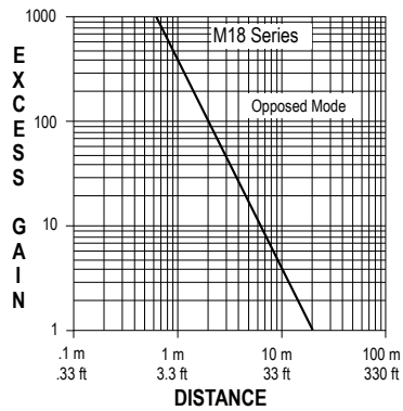
Excess Gain
