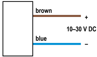
Figure 8. Emitters with Attached Cable
