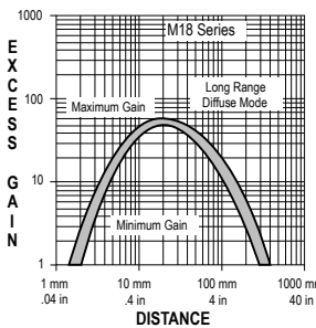
Excess Gain
