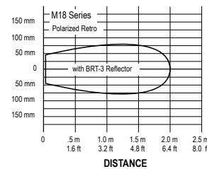
Beam Pattern
