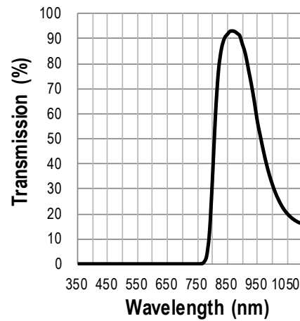
Figure 2. Percent Transmission of light wavelengths through FLTMI infrared filter
