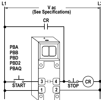
Figure 10. Wiring in Series with Contacts or Switches
