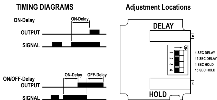
Figure 2. Timing Diagrams and Adjustment Locations
