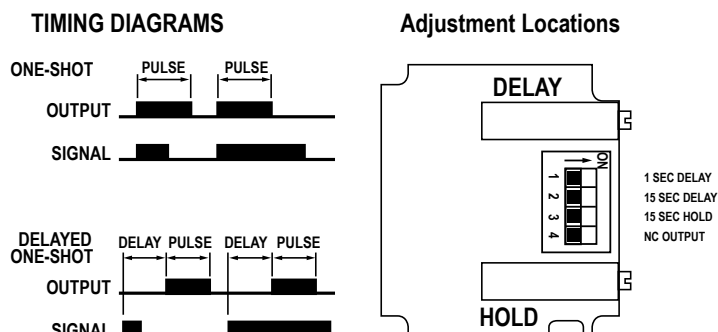
Figure 3. Timing Diagrams and Adjustment Locations
