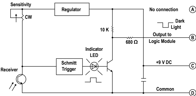
Figure 1. Functional schematic
