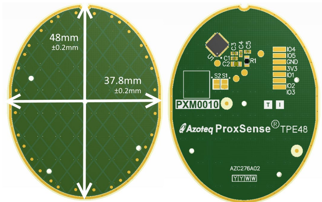
Figure 6-1: TPE48 – Front and Back View.
