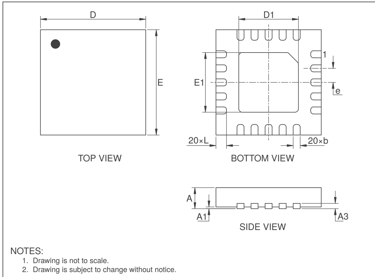
Figure 15.1: QFN (3x3)-20 (QFR) Package Outline Visual Description
