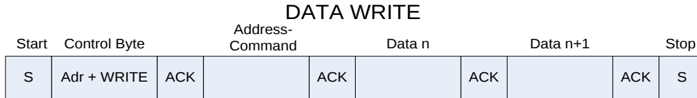
Figure 8.4 I2C Write
