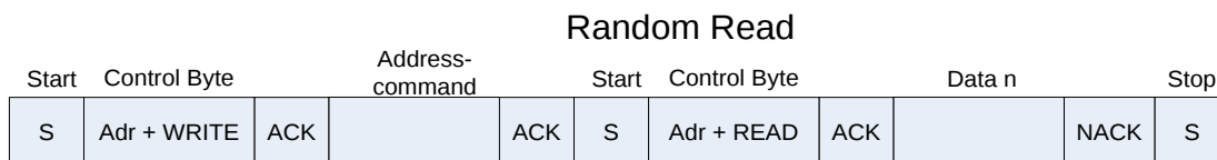
Figure 8.3 Random Read
