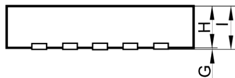
Figure 10.2 DFN(3x3)-10 Package dimensions (side view)
