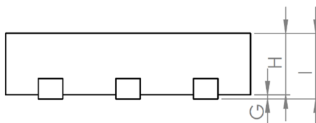
Figure 12.3 DFN-6 Package Dimensions (side)
