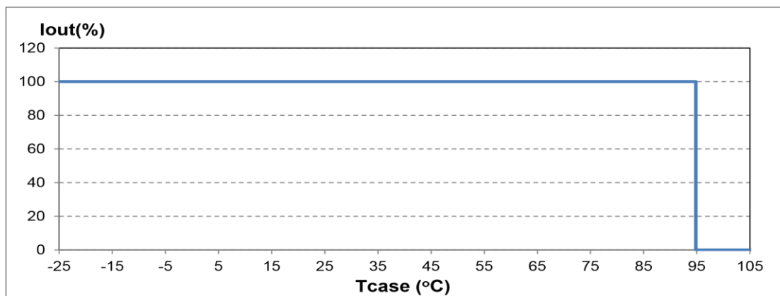
Output Current vs. Case Temperature (with ±5°C Tolerance)
