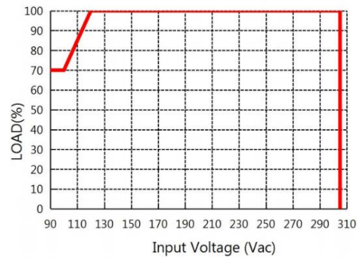
Fig. 7 Output Power VS Input Voltage
