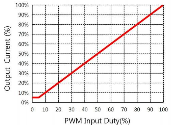
Fig. 9 PWM Dimming Curve
