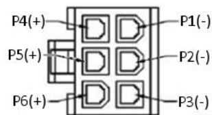
Output Cable Plug Pin Assignment
