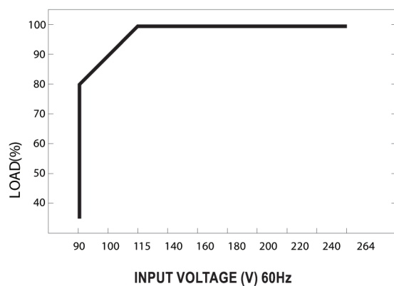
■ Static Characteristics (MPS-200)
