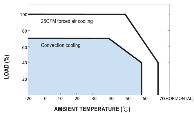
■ Derating Curve (MPS-200)
