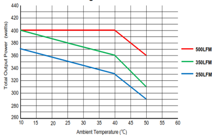
Power Rating at 100Vac for 12V
