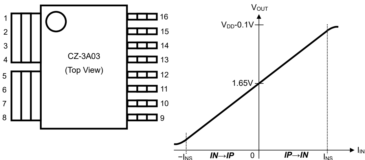
Figure 2. Pin configurations and typical output characteristics of CZ-3A03
