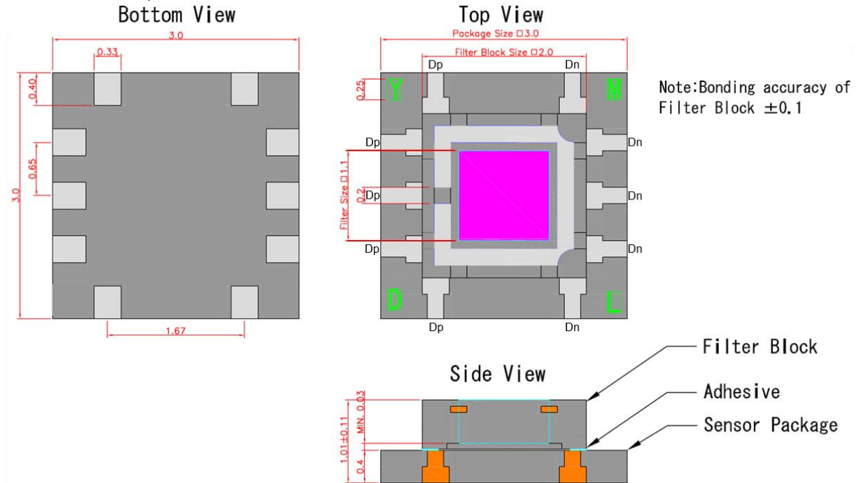
Figure 12.1 Outline Dimensions
