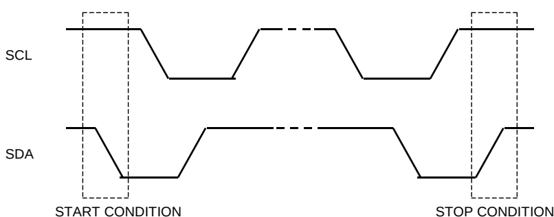
Figure 7.2. Start and Stop Condition
