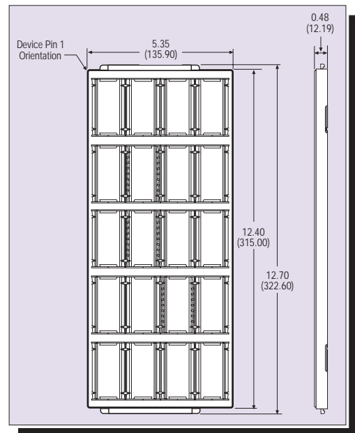
Figure 10 - Matrix Tray Dimensions
