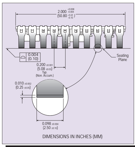
Figure 9 - Dimensioned Product View
