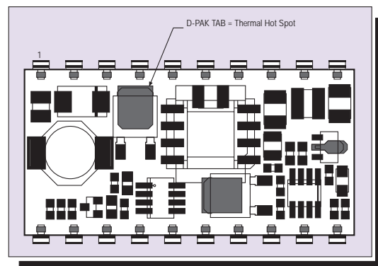
Figure 7 - Thermal Hot Spot
