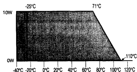
DERATING CURVE (See Note 8) Output Power (Watts)
